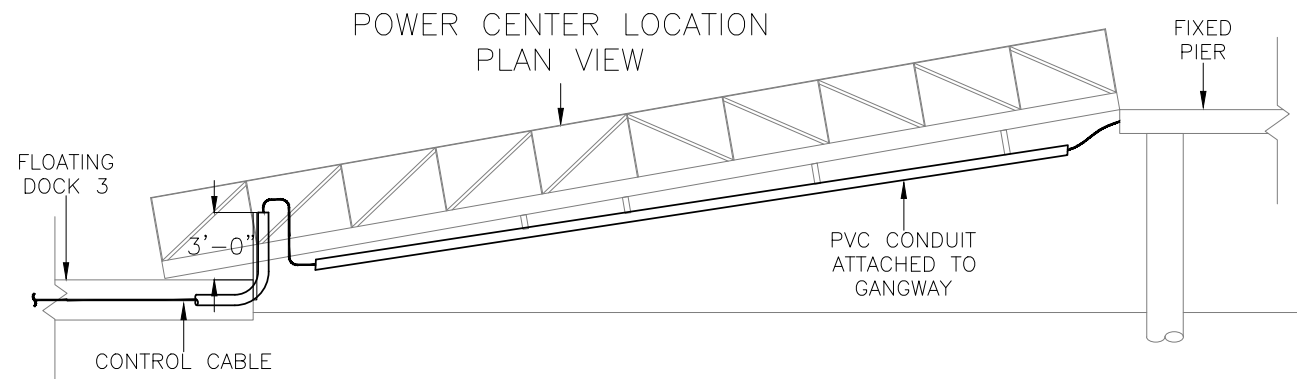
CONTROL CABLE GANGWAY TO FLOATING DOCK DETAIL NOT TO SCALE
